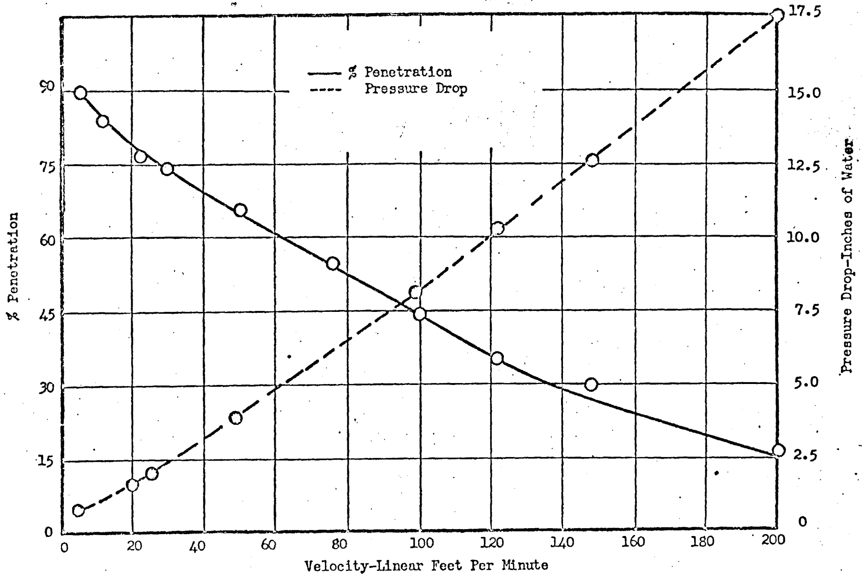
DOP SMOKE PENETRATION AND PRESSURE DROP VERSUS VELOCITY FOR WHATMAN NO. 41 PAPER
