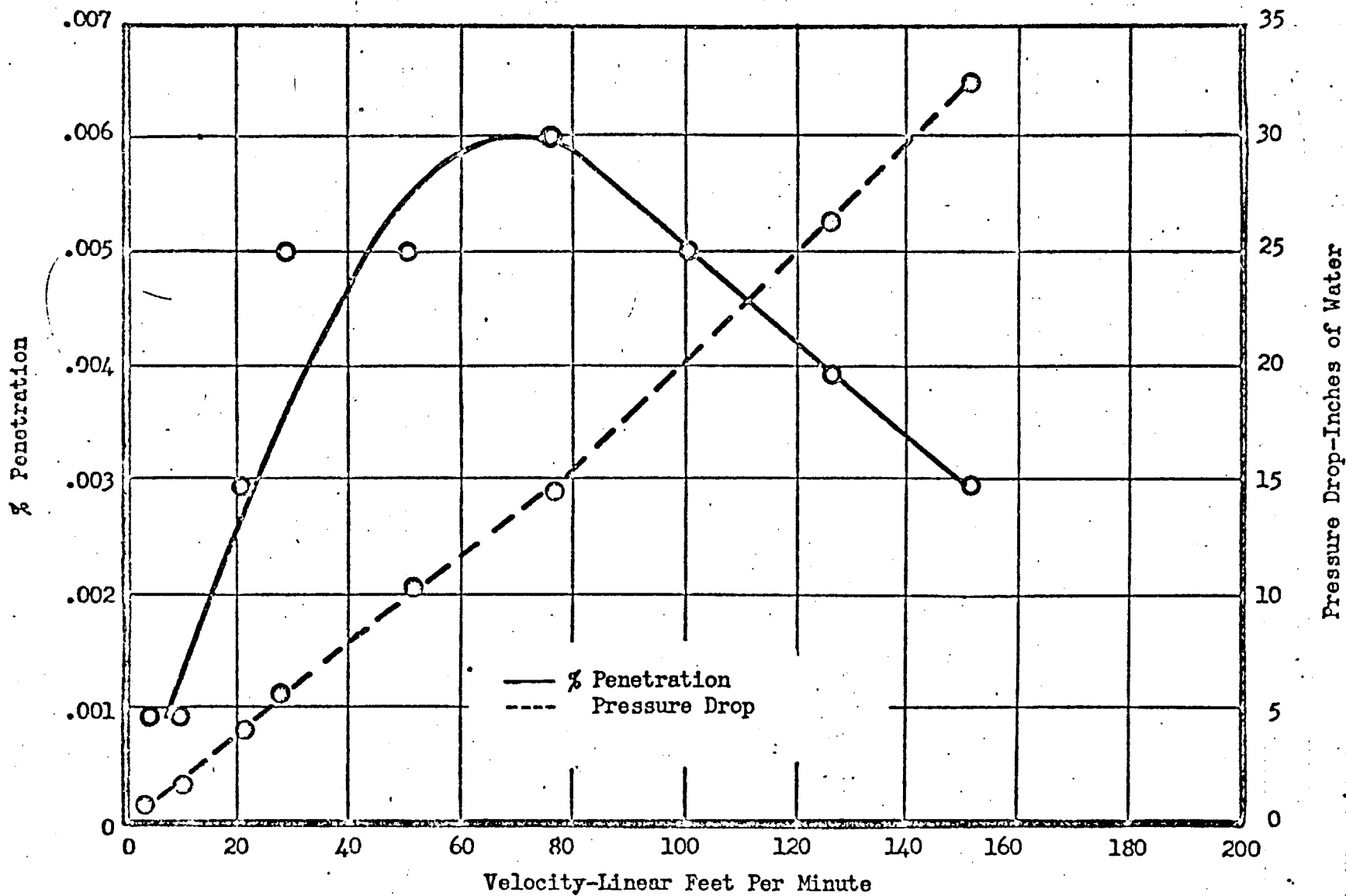
DOP SMOKE PENETRATION AND PRESSURE DROP VERSUS VELOCITY FOR HURLBUT GLASS FIBER PAPER
