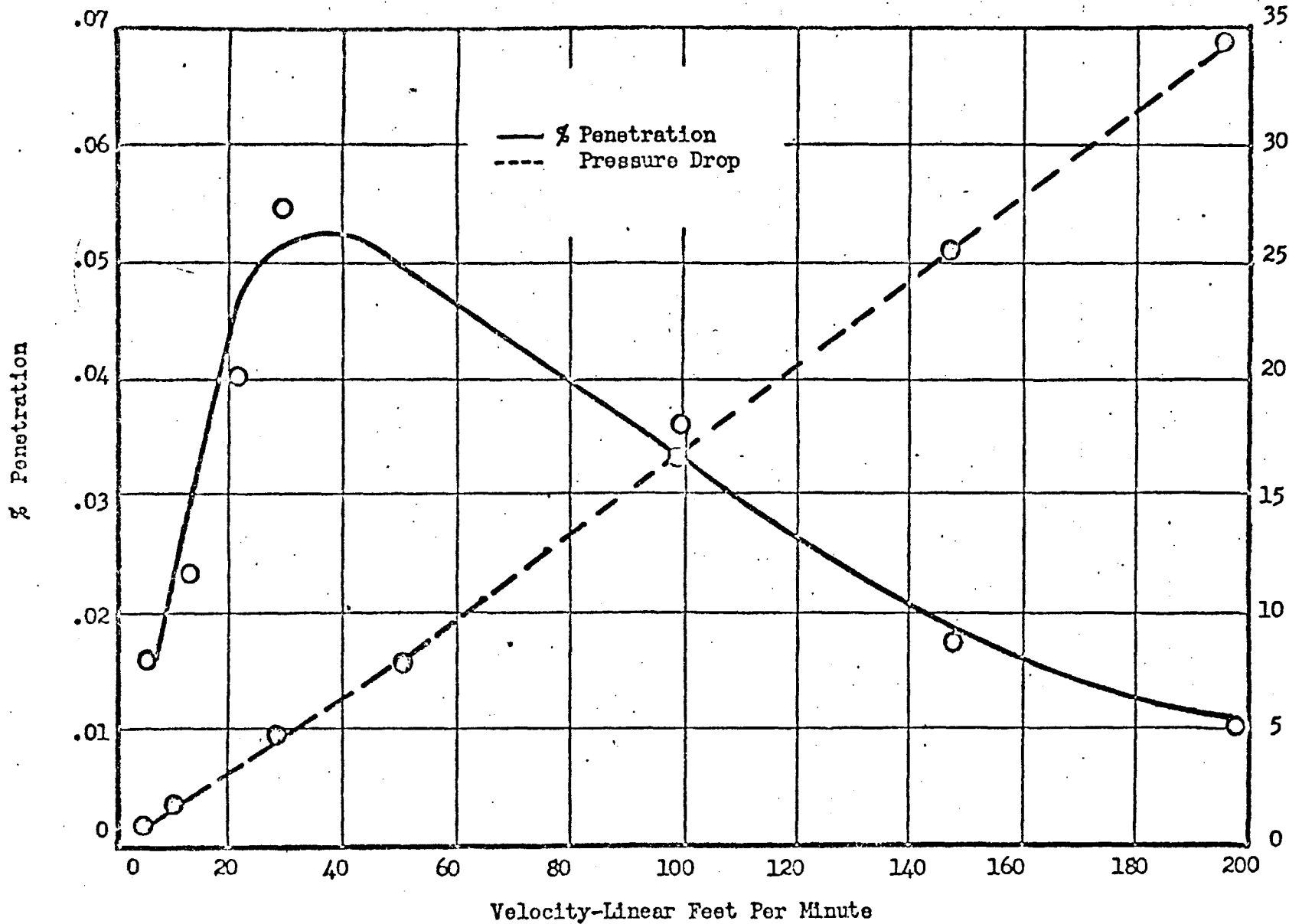
DOP SMOKE PENETRATION AND PRESSURE DROP VERSUS VELOCITY FOR C.W.S. NO. 6 PAPER
