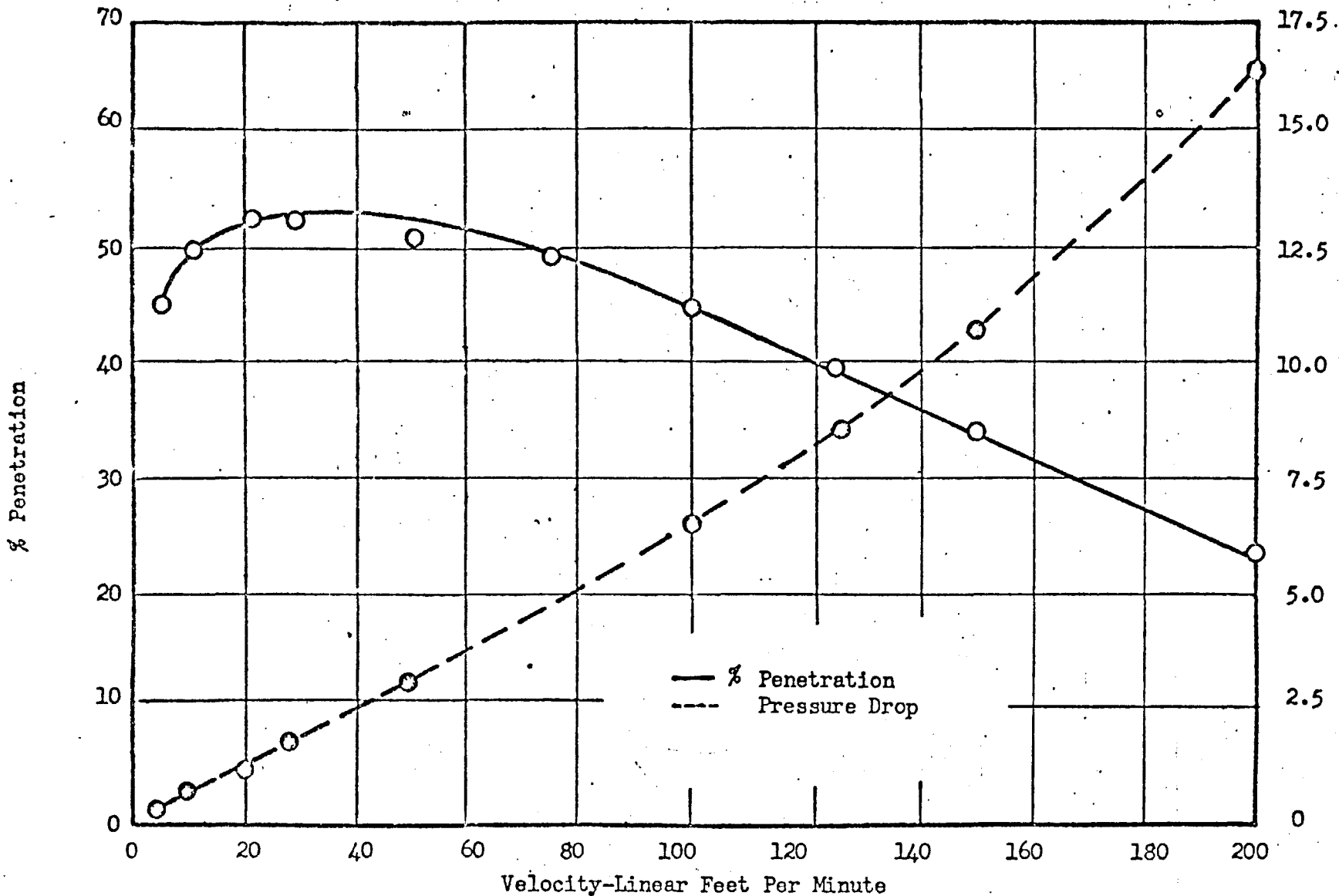
DOP SMOKE PENETRATION AND PRESSURE DROP VERSUS VELOCITY FOR M.S.A. TYPE "S" FILTER
