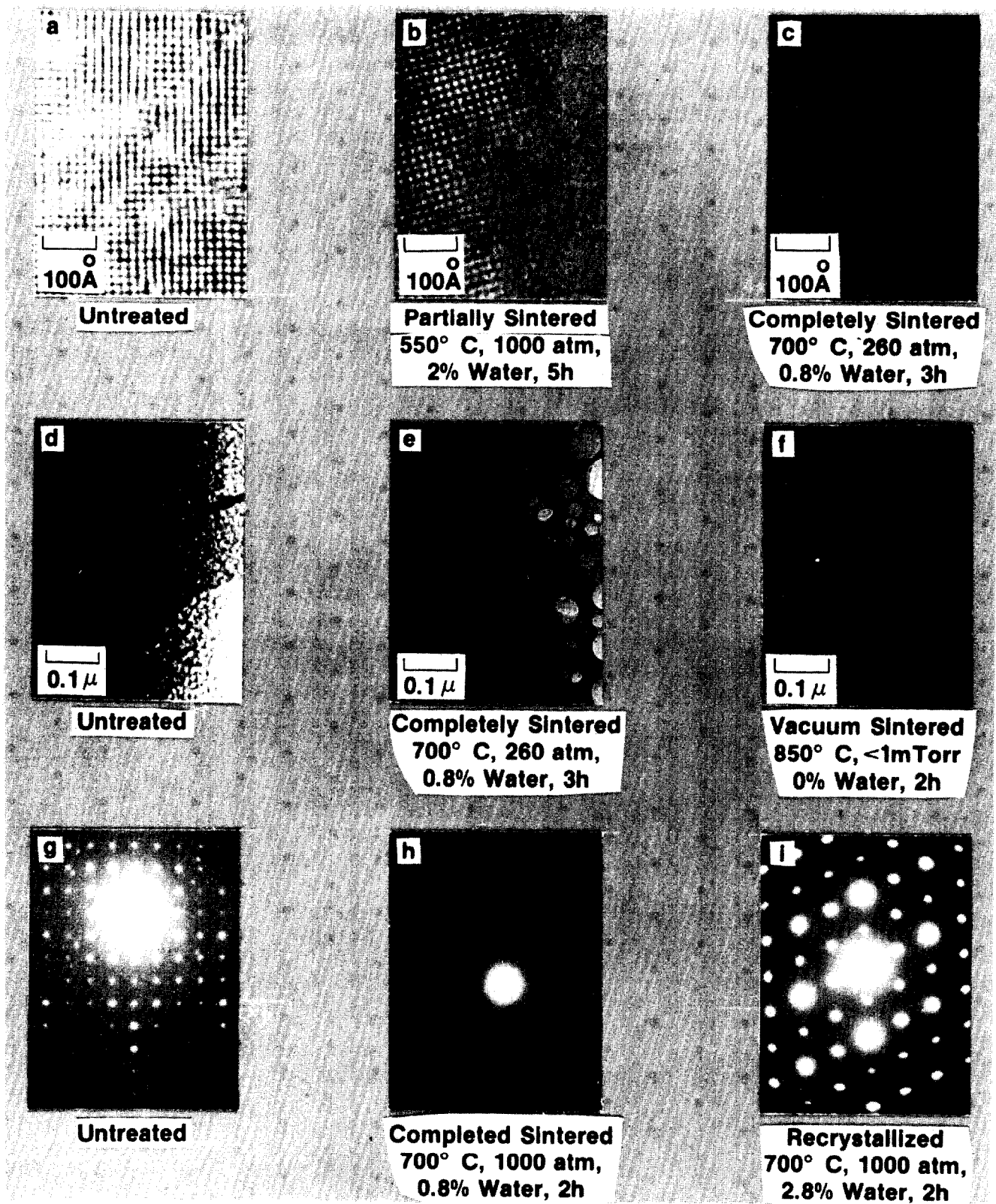
Figure 7. Electron Micrographs and Electron Diffraction Patterns of Zeolite 5A.
