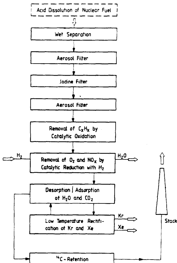
Fig. 5: Scheme for off-gas cleaning for a fuel reprocessing plant for LWR
