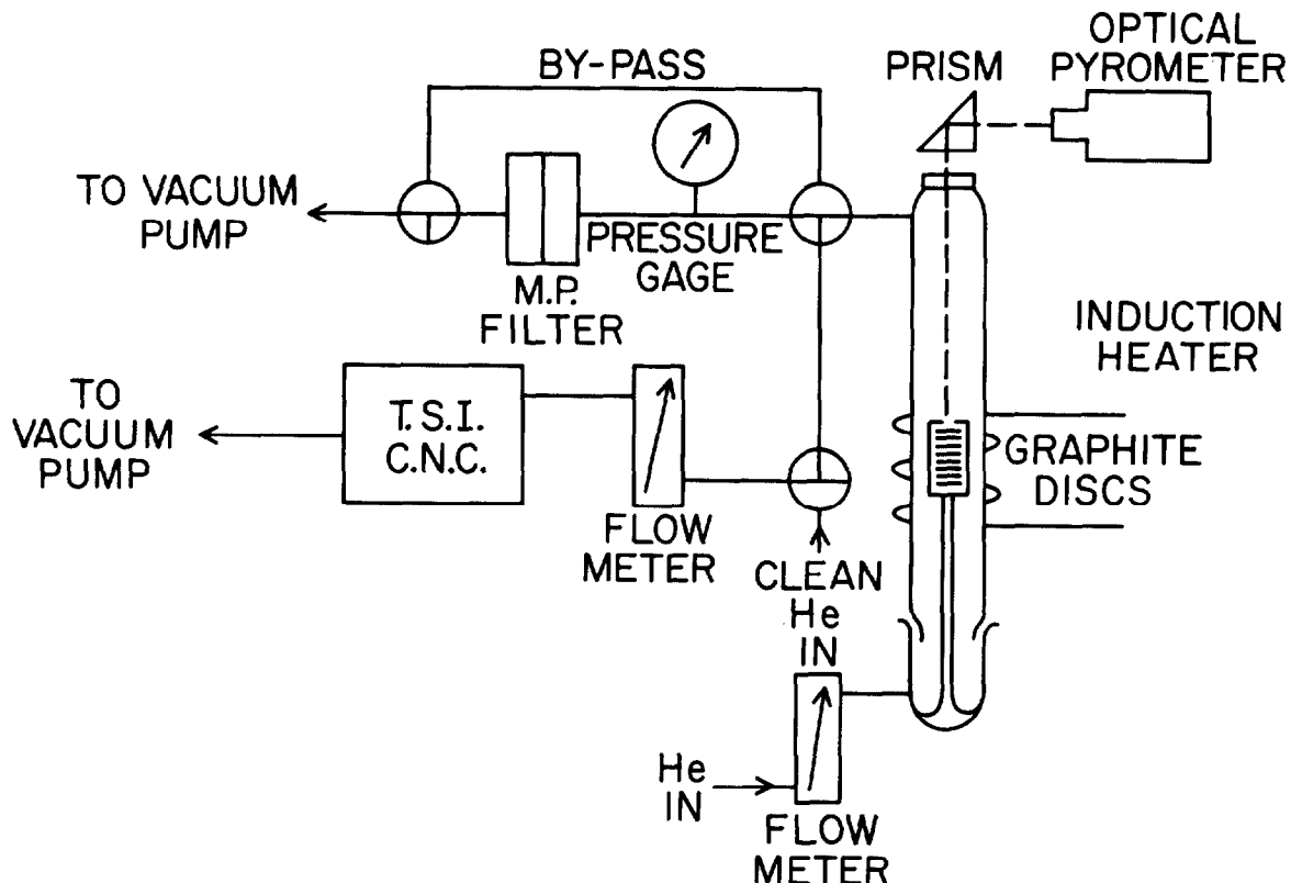
Figure 1. Schematic Diagram of Fission Product Transport Apparatus
