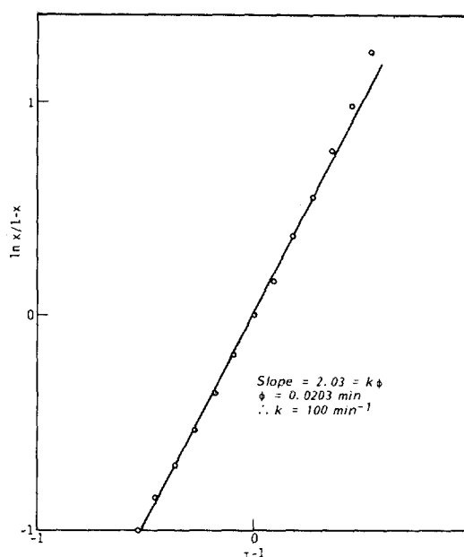
FIGURE 3 DETERMINATION OF REACTION ORDER AND RATE CONSTANT
