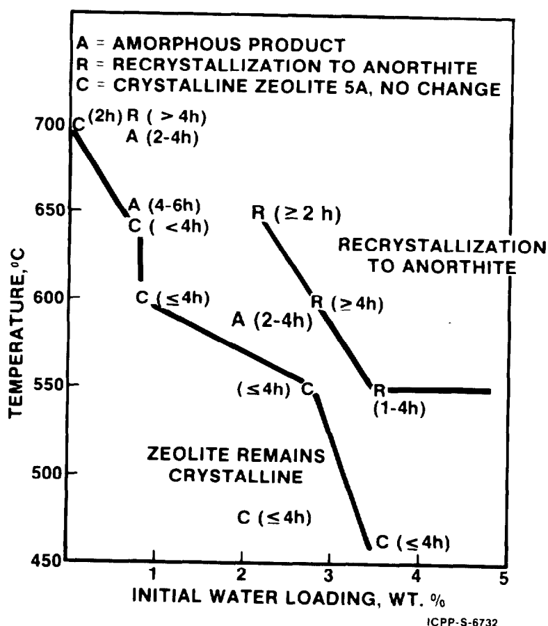
Figure 5. Effect of Encapsulation Temperature, Time, and Initial Water Loading on the Product Formed from Grace-Davison Zeolite 5A.
