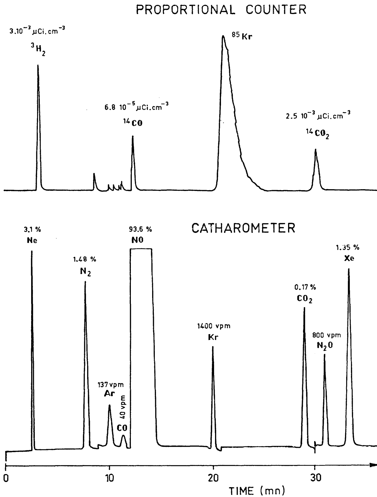
Figure 3 : Typical chromatogram
