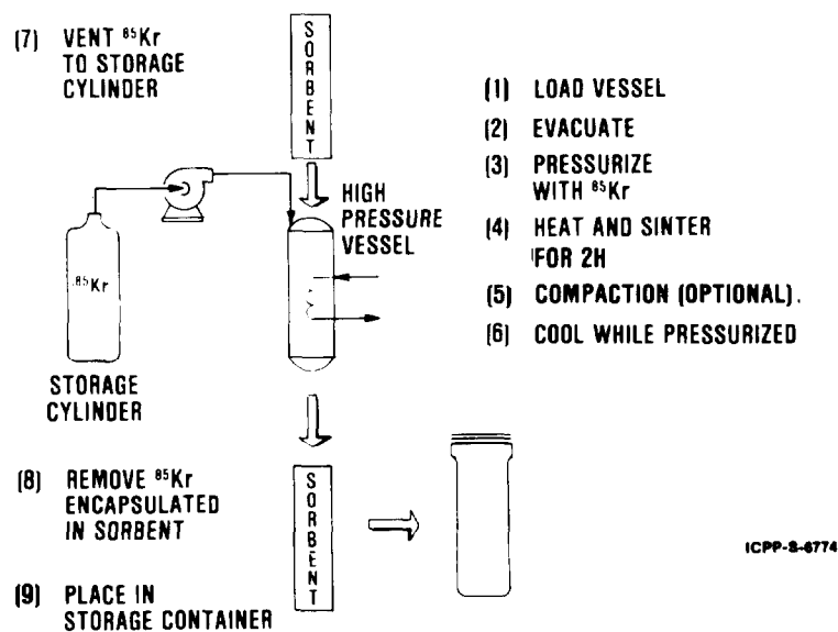
Figure 1. Schematic of the Process Used to Encapsulate Krypton by Sintering in Zeolite 5A.
