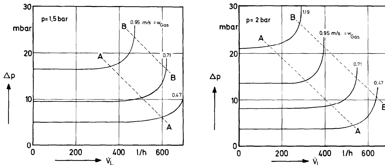
Fig. 13: Pressure drop \Delta p in dependence of the caustic solution flow rate \dot{V}_L
