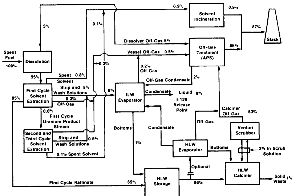
FIGURE 10. ^{129}\text{I} TRANSPORT THROUGH FUEL REPROCESSING PLANT WITHOUT HLW EVAPORATION
