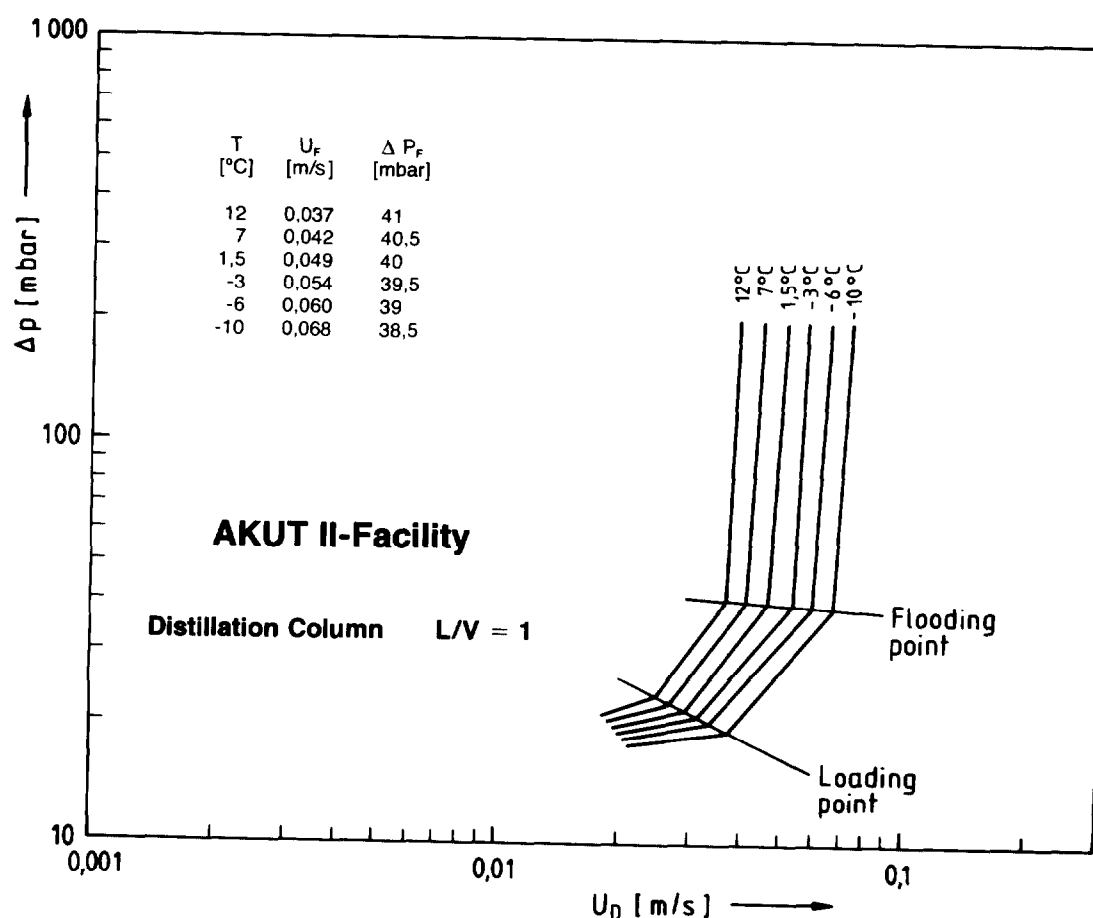
Figure 4: The Pressure Drop \Delta p through the Distillation Column versus Vapor Velocity U_D at Various Temperatures
