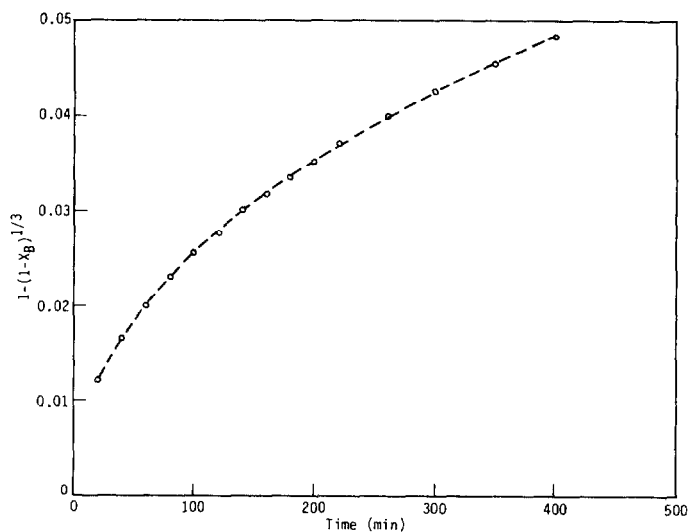
FIGURE 9 DETERMINATION OF RATE CONTROLLING STEP FOR LOW HUMIDITY EXPERIMENT (G640) (ASSUMING CHEMICAL REACTION CONTROLLED)
