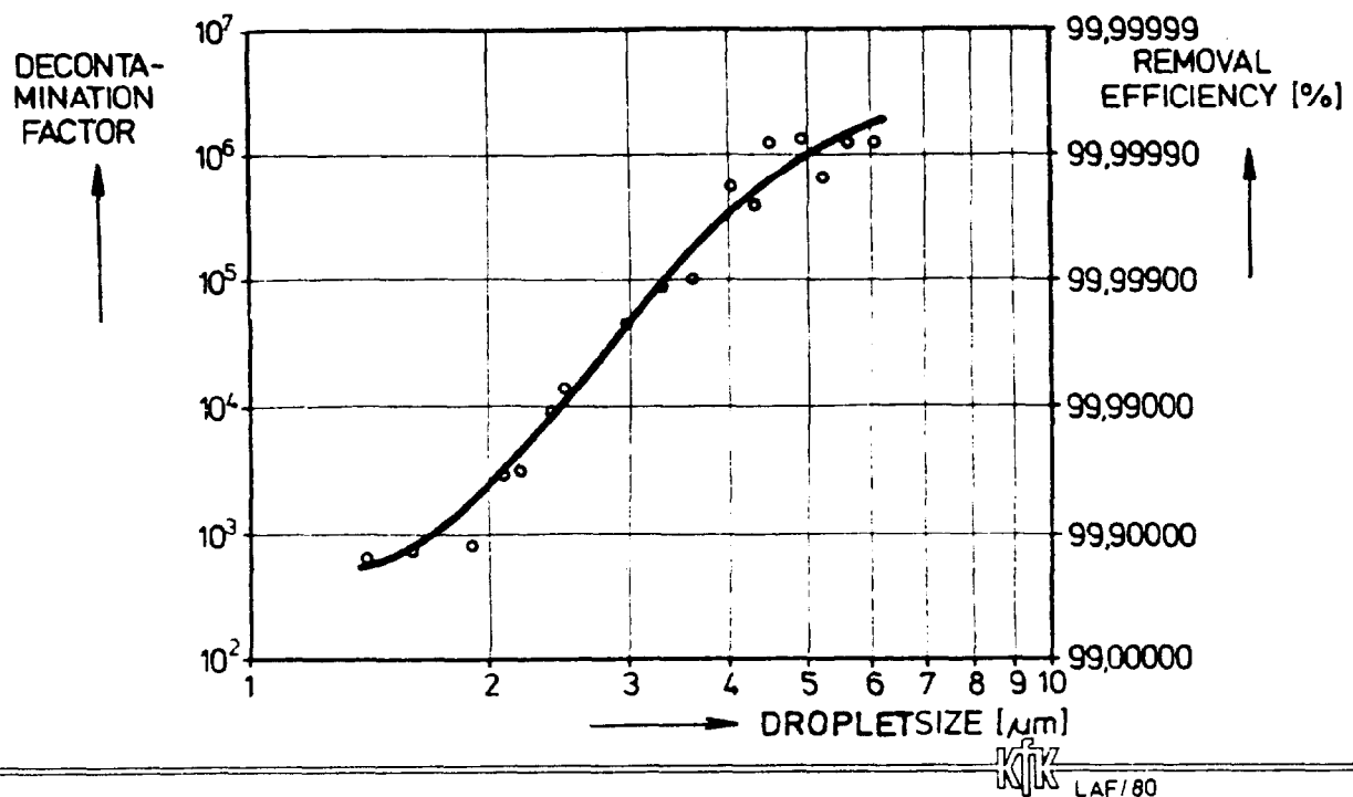
FIG. 4: DECONTAMINATION FACTOR AS A FUNCTION OF DROPLET SIZE (PFME/ 5 cm)
