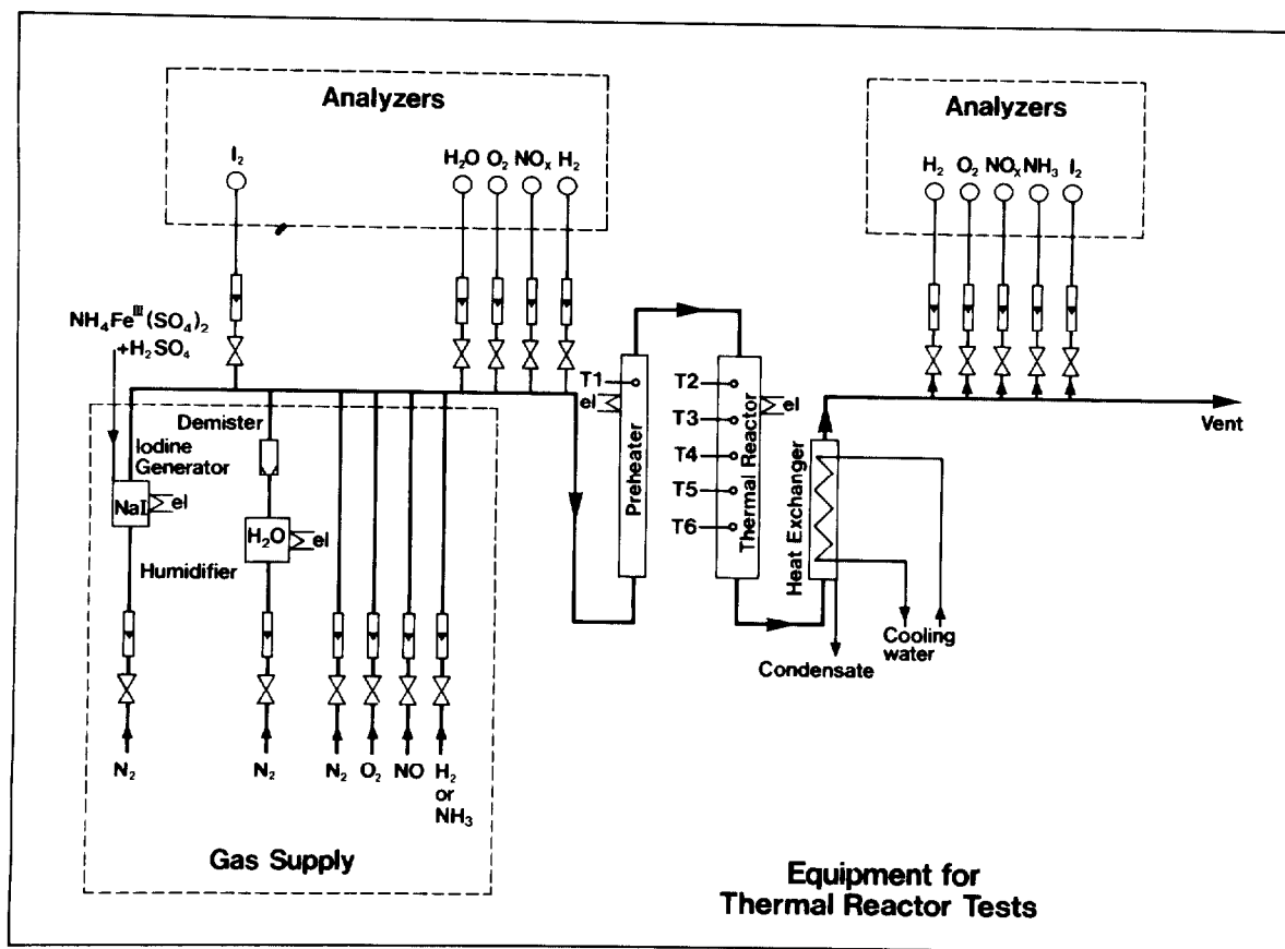
Figure 6: Test Assembly
