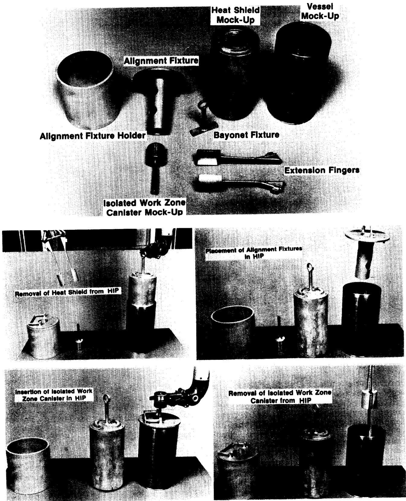
Figure 14. Mock-up of Lab-Scale HIP Components and Tools Required for Remote Operations
