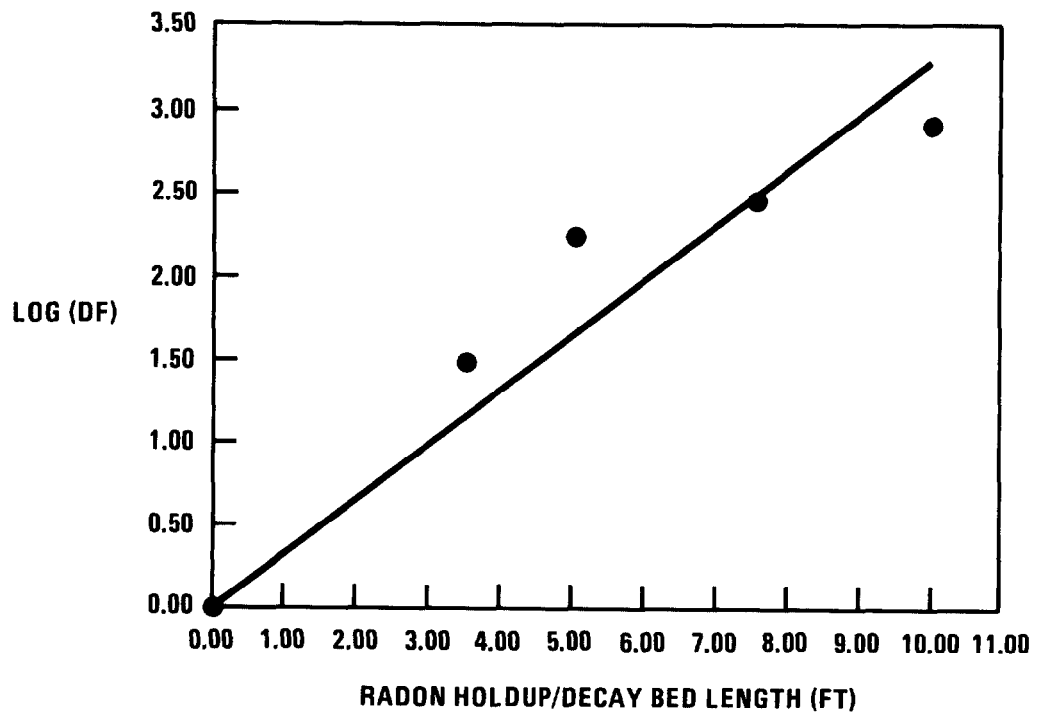
Figure 16. Plot of log DF versus radon holdup/decay bed length.
