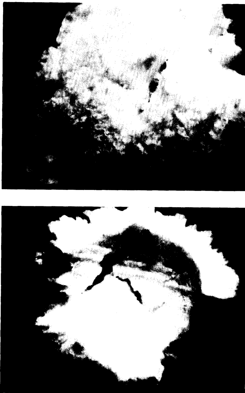
Fig. 7. Top and bottom views of a commercial \text{Ba}(\text{OH})_2 \cdot 8\text{H}_2\text{O} flake subjected to relative humidity >60\% .
