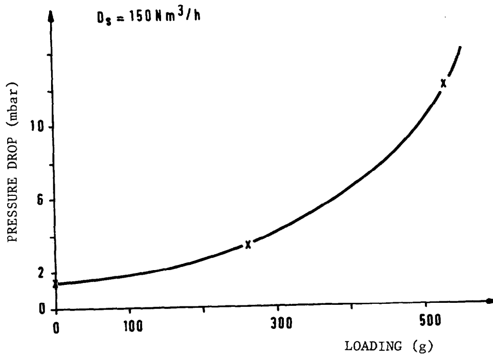
Fig. 8: PRESSURE DROP OF THE HEPA-FILTER AS A FUNCTION OF LOADING
