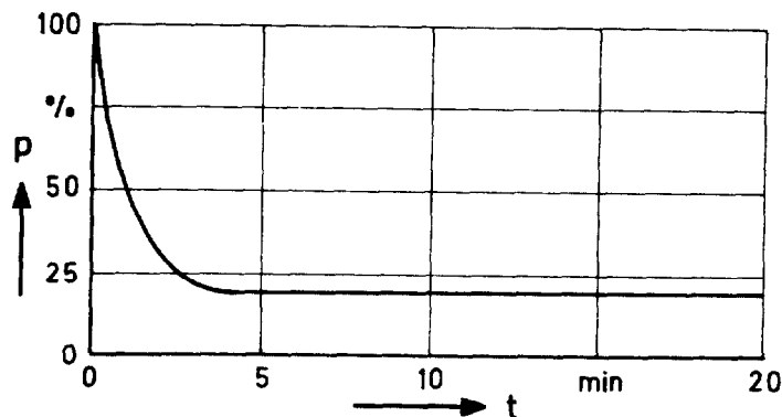
Fig. 14: Conversion in the compression zone, if 1 l poudorous 0.5 mol \text{Ca}(\text{OH})_2 is added to 0.5m \text{Na}_2\text{OH} -solution ans is mixed for 1 minute
