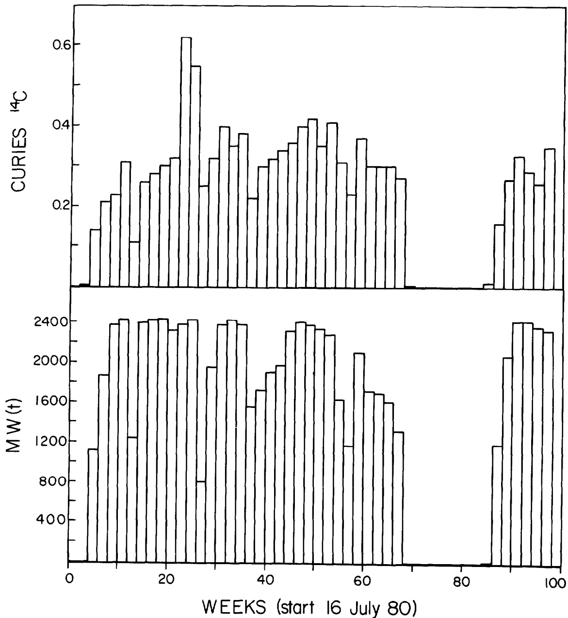
Figure 7 Biweekly measurements of 14 C discharge from off-gas stack and average power levels of an 850 MW(e) BWR.
