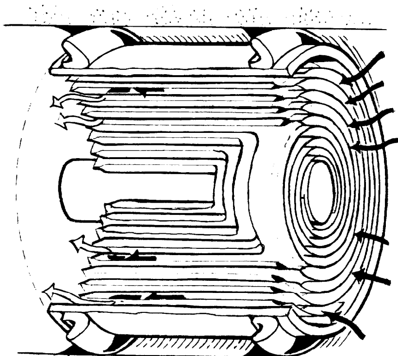
FIGURE 12 AIR-FLOW DISTRIBUTION WITHIN AN AXIAL-FLOW CIRCULAR
