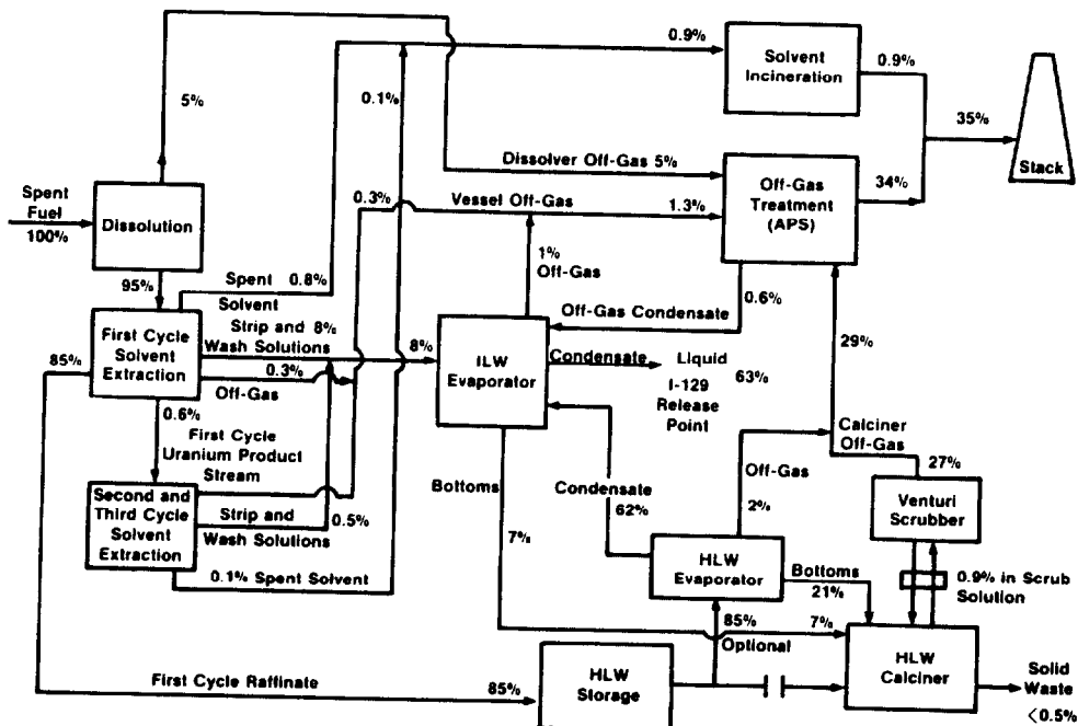
FIGURE 11. ^{129}\text{I} TRANSPORT THROUGH FUEL REPROCESSING PLANT WITH HLW EVAPORATION
