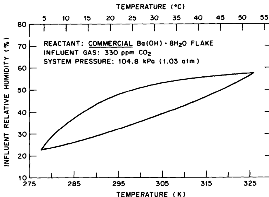
Fig. 11. Operating window for contacting a 330-ppmv \text{CO}_2 gas stream with fixed beds of commercial \text{Ba}(\text{OH})_2 \cdot 8\text{H}_2\text{O} flakes under isothermal conditions.
