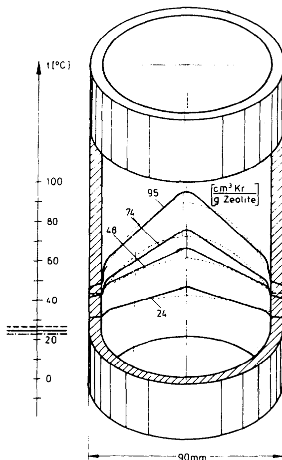
Fig. 3 Temperature profile in a 90 mm \varnothing cylinder as a function of zeolite loading with radioactive krypton. The dotted lines correspond to temperatures calculated with thermal conductivity values obtained in this work.
