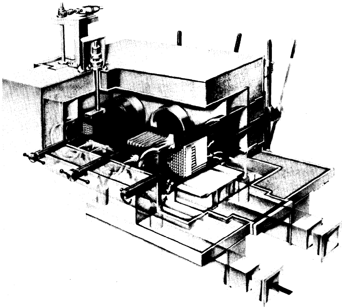
FIGURE 2 FILTER HOUSING
