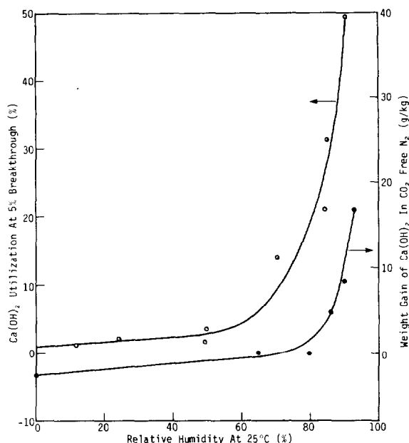
FIGURE 7 THE EFFECT OF HUMIDITY ON THE WEIGHT GAIN AND UTILIZATION OF \text{Ca}(\text{OH})_2
