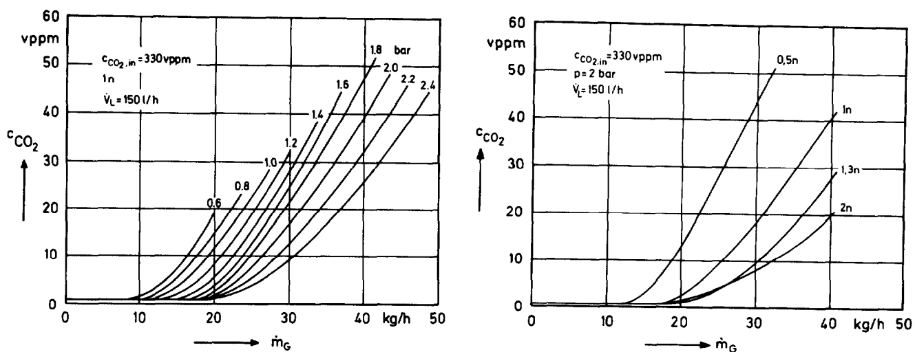
Fig. 10: CO 2 off-gas concentration c_{CO_2} in dependence of the gas flow rate \dot{m}_G , the pressure and the caustic solution concentration at a constant feed concentration of 330 vppm
