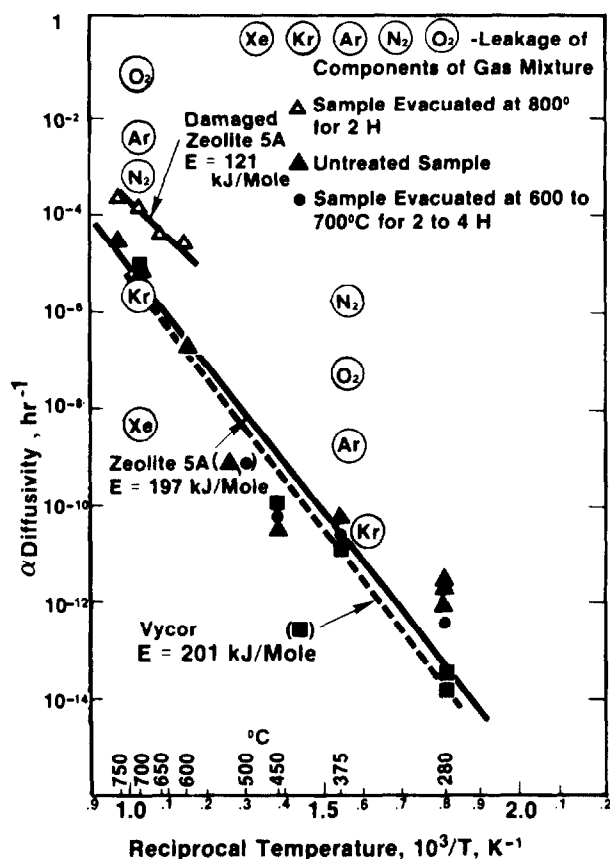
Figure 10. Temperature Dependence of Diffusivity of Krypton from Sintered Zeolite 5A.
