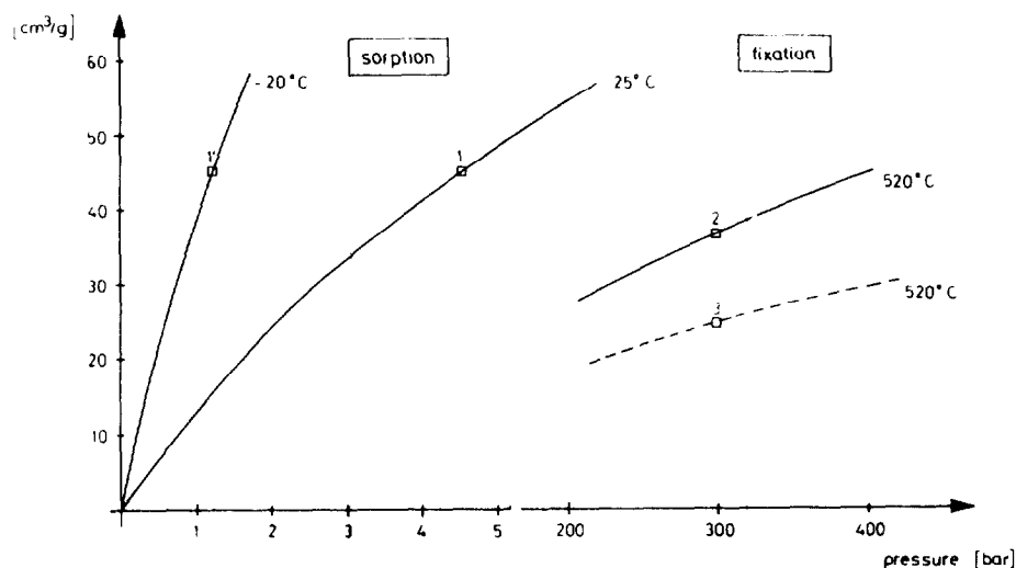
Fig. 6 Sorption and fixation isotherms for krypton in zeolite 5A
