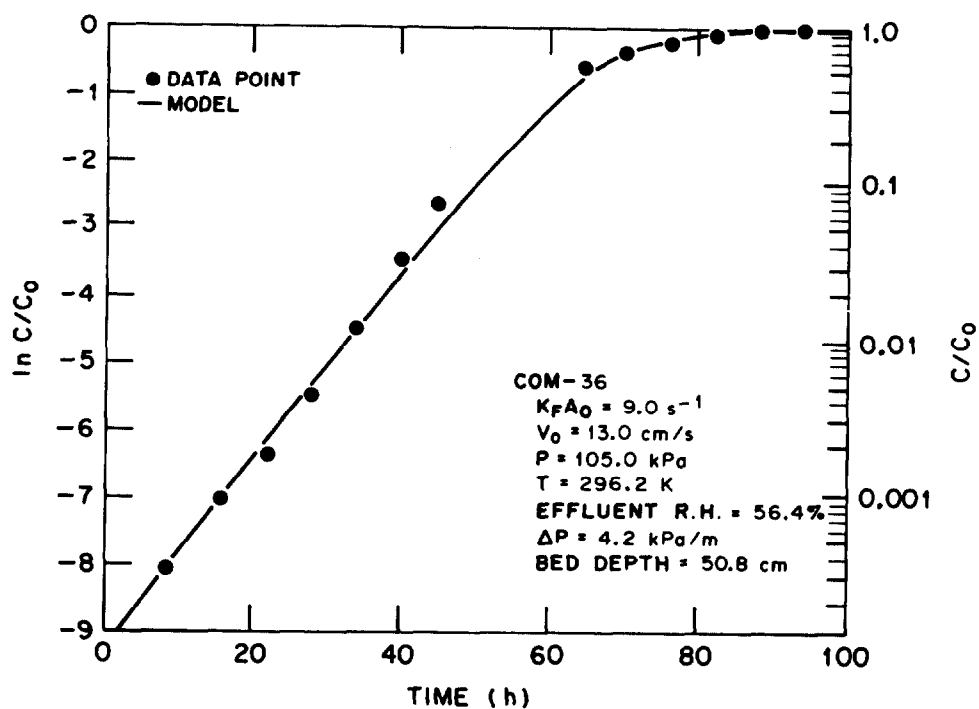
Fig. 8. Breakthrough curves and model-predicted breakthrough curves for typical fixed-bed runs.
