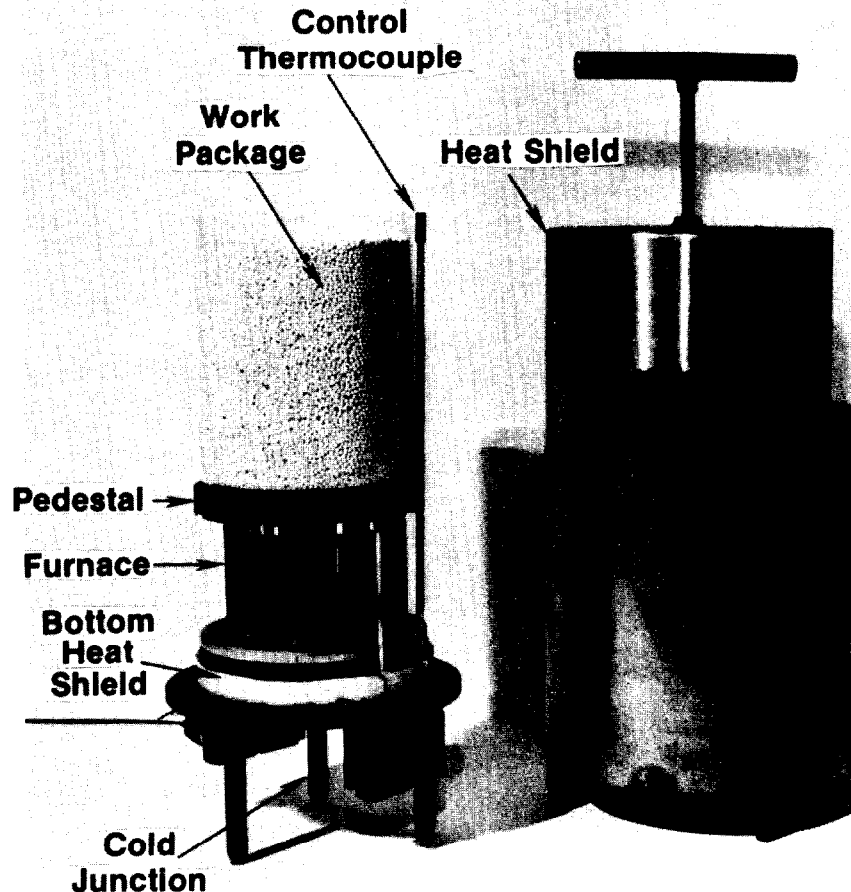
Figure 4. Interior Components of the Laboratory-Scale HIP.
