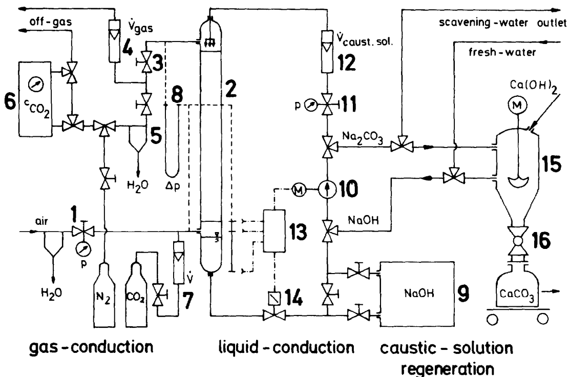
Fig. 8: Flow sheet of the experimental set-up for CO 2 -separation
