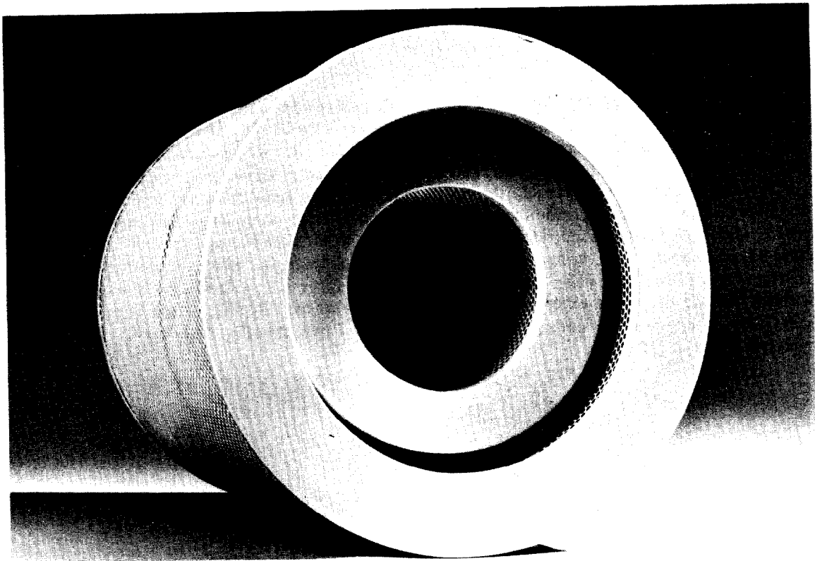
FIGURE 8 EXTENDED LIFE RADIAL FLOW CIRCULAR FILTER RATED AT 1700\text{ m}^3/\text{h}
