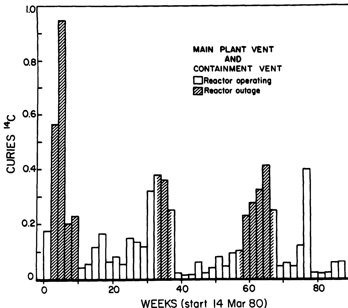
Figure 4 Combined ^{14}\text{C} discharge from main plant vent and containment vent of a 490 MW(e) PWR.
