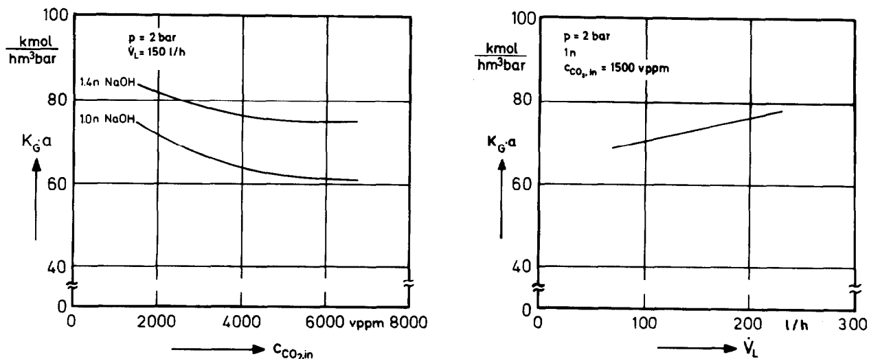
Fig. 12: Mass transfer constant K_G \cdot a in dependence of the feed concentration c_{CO_2} , the caustic solution flow rate \dot{V}_L and the caustic solution concentration
