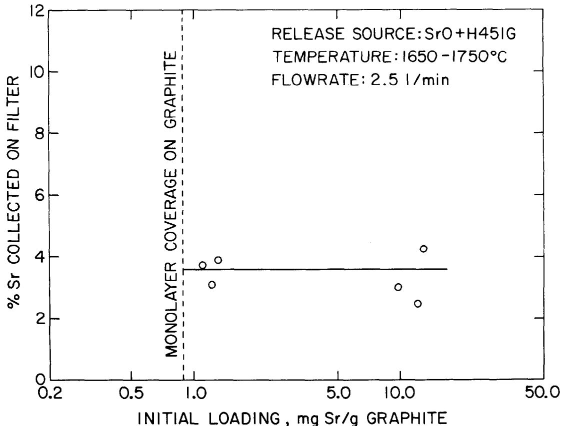
Figure 6. Effect of Initial Sr Loading on Particulate Transport
