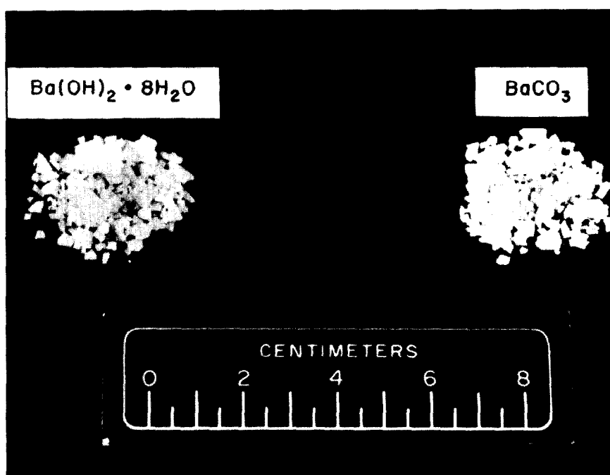
Fig. 1. Commercial \text{Ba(OH)}_2 \cdot 8\text{H}_2\text{O} flaked reactant and \text{BaCO}_3 flaked product. The product was obtained at a process relative humidity <60%.
