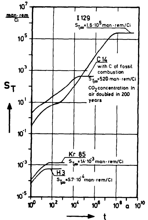
Fig. 4: Total collective effective dose equivalent commitment S_T from globally distributed radionuclides in dependence of integration time (world population 1 \cdot 10^{10} )
