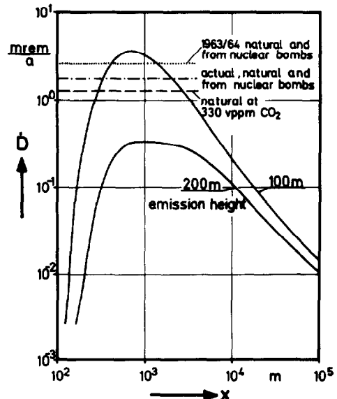
Fig. 2: Maximum radiation exposure due to ^{14}\text{C} of an adult in main wind direction (east), \dot{E} = 500 \text{ Ci/a}
