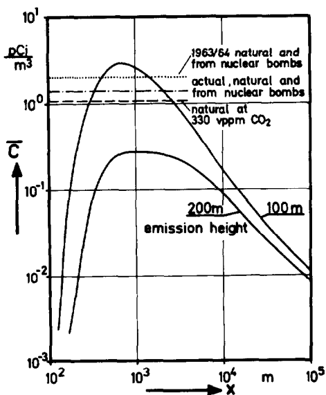
Fig. 1: ^{14}\text{C} concentration of the air near ground level in the main wind direction (east), \dot{E} = 500 \text{ Ci/a}
