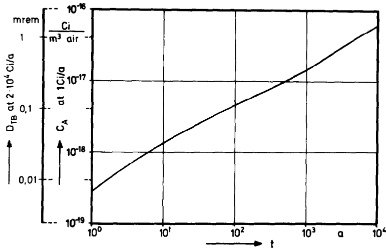
Fig. 3: ^{14}\text{C} activity in the air at ground level after global distribution, if 1 Ci ^{14}\text{C} is emitted per year; total body annual dose for an annual emission of 2 \cdot 10^4 Ci without ^{14}\text{C} -concentration changes due to nuclear weapon tests; \text{CO}_2 concentration in the air 330 vppm = const.
