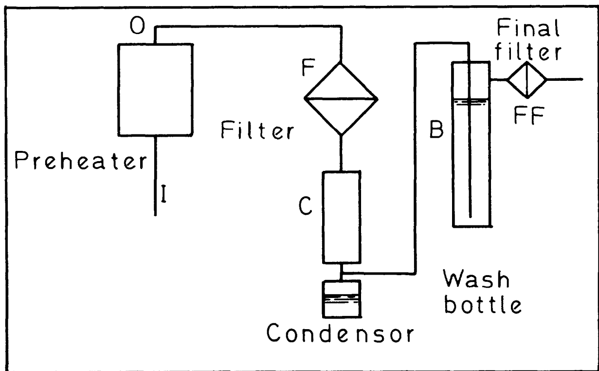
Fig. 3. Modified installation for the study of the influence of the preheating temperature
