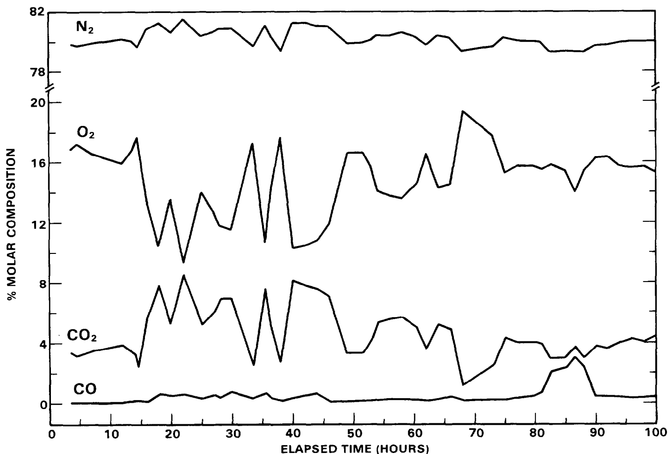
Figure 3. Combustion boosted melter exhaust composition.
