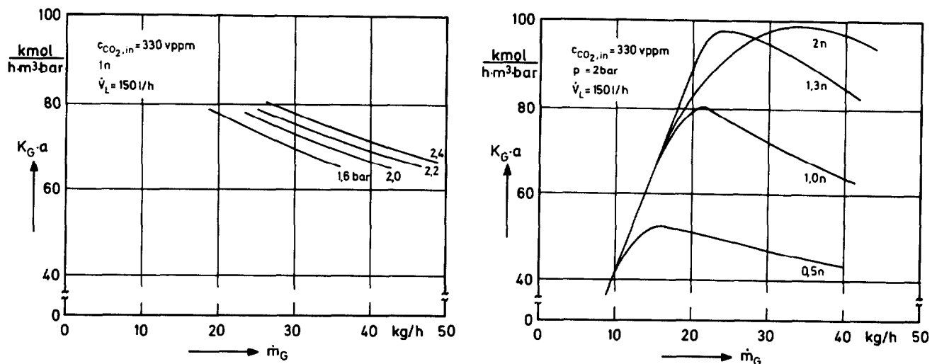
Fig. 11: Mass transfer constant K_G \cdot a in dependence of the gas flow rate \dot{m}_G , the pressure and the caustic solution concentration at a constant feed concentration of 330 vppm
