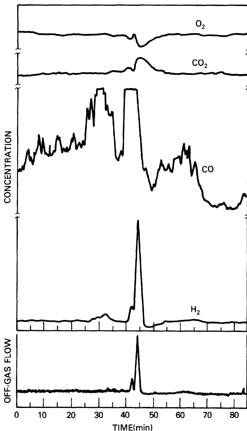
Figure 5. Compositional behavior of noncondensable melter exhaust gases accompanying a flow surge. (Maximum extent of the surge event: flow-3X; H_2 < 3.5\% ; CO \gg 0.5\% ; CO_2 - 15\% ; O_2 - 17\% .)
