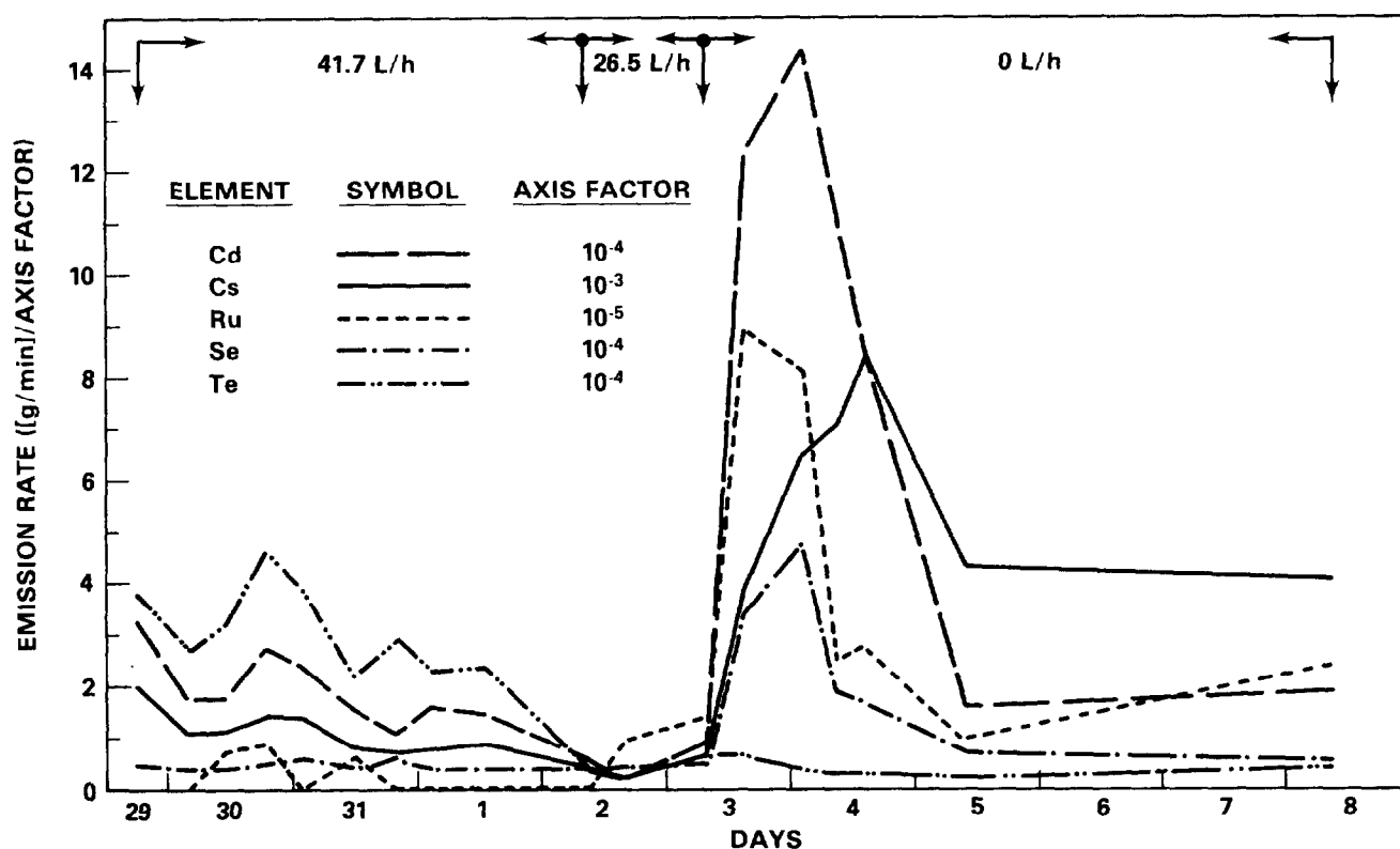
Figure 8. Melter idling emission rates of semivolatile elements.
