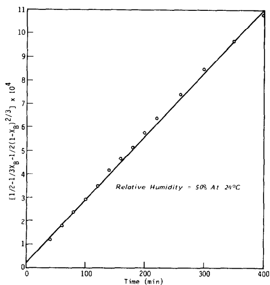
FIGURE 8 DETERMINATION OF RATE CONTROLLING STEP FOR LOW HUMIDITY EXPERIMENT (G640) (ASSUMING DIFFUSION THROUGH PRODUCT LAYER CONTROLLED)
