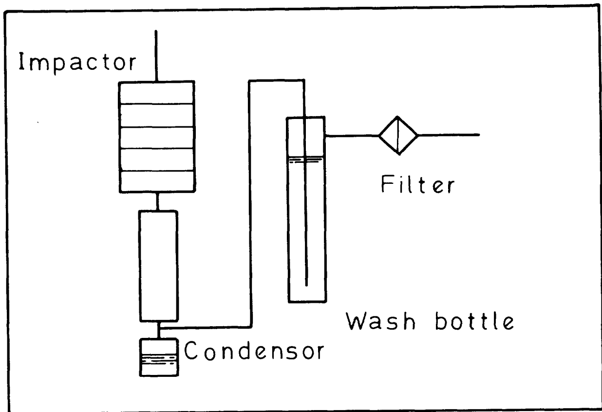
Fig. 2. Flow sheet of the sampling unit
