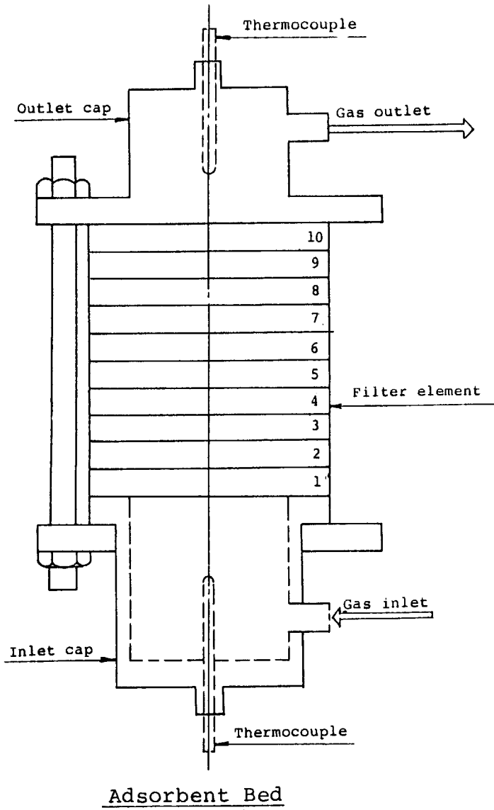
Fig.2 Filter Element and Filter Bed Assembly
